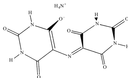
Fig. 1 Structure of murexide
