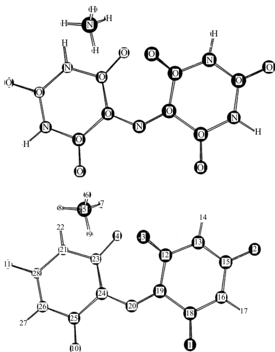
Fig. 2 The postulated structure of murexide
