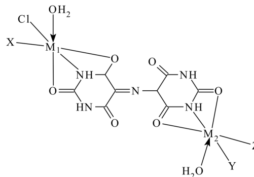
Fig. 3 The structures of all murexide complexes except IX where Complex I when there is no M_2 and M_1=Fe , X=Cl . Complexes III , V , VII , X and XI when there is no M_2 , X=H_2O and M_1=Co , Ni , Cu and Cd , respectively. Complex II M_1= M_2=Fe and X=Y=Z=Cl . Complexes IV , VI and VIII when, X=H_2O , Y=Z=Cl and M_1=M_2=Co , Ni and Cu , respectively
